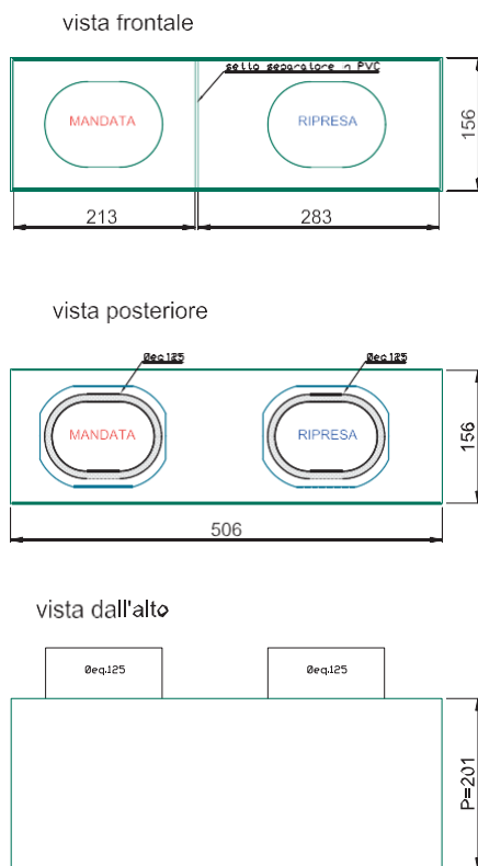
Drawing of COMBIPL 500x150 mm plenum with custom \varnothing_{eq} 125mm connections.
