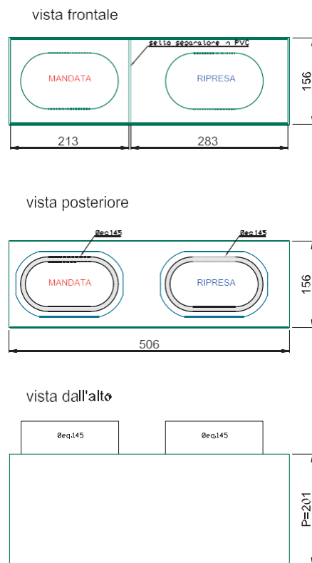
Drawing of COMBIPL 500x150mm plenum with standard \varnothing_{eq} 145mm connections.
